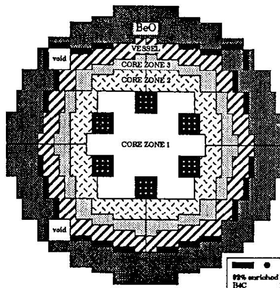
ZPPR-16B CONTROL WORTH MEASUREMENTS
