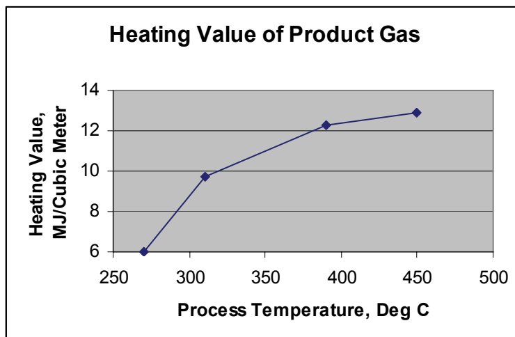
FIGURE 7.1 Heating Value of the Product Gas as a Function of Temperature (based on the data of Horii and Iida 2001)
