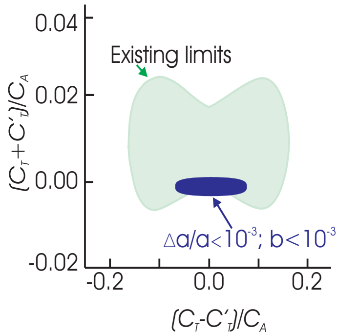
Figure 7-2. 95% confidence intervals: presently allowed region (from Ref. [145]) in green and, in blue, the limits one would get with measurements of \Delta a/a < 10^{-3} and \Delta b < 10^{-3} .
