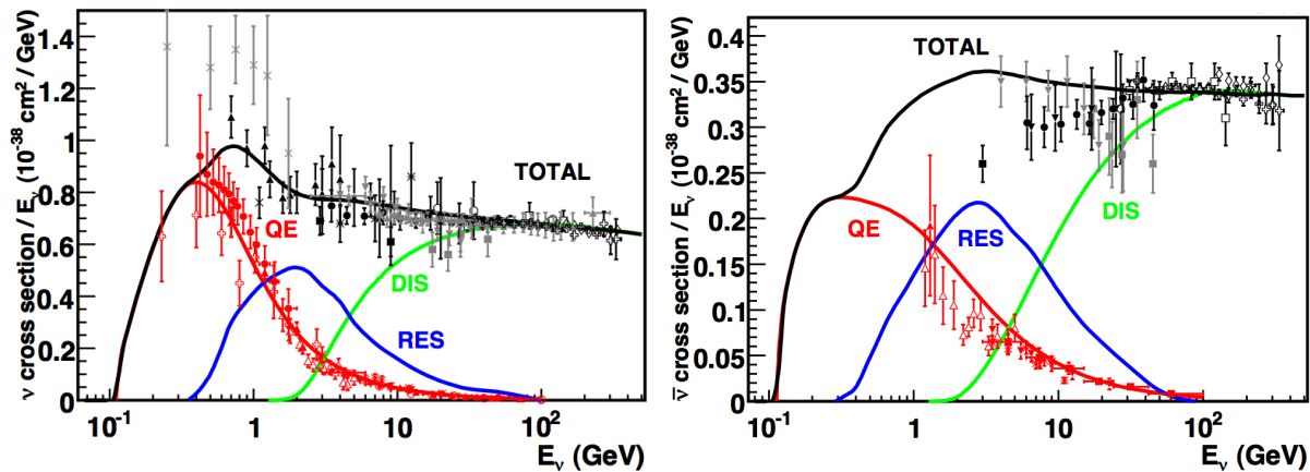
Figure 4-8. Existing muon neutrino (left) and antineutrino (right) charged-current cross section measurements [?] and predictions [?] as a function of neutrino energy. The contributing processes in this energy region include quasi-elastic (QE) scattering, resonance production (RES), and deep inelastic scattering (DIS). The error bars in the intermediate energy range reflect the uncertainties in these cross sections (typically 10 – 40%, depending on the channel).
