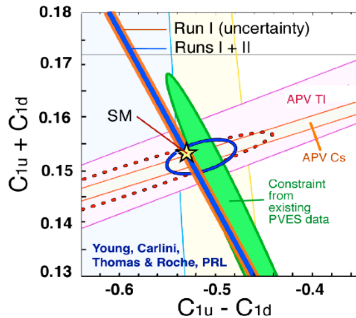
Figure 7-5. Knowledge of the neutral-weak effective coupling constants. The dotted contour displays the previous experimental limits (95% CL) reported in the Particle Data Group Review[173] together with the prediction of the standard model (yellow star). The filled ellipse denotes the present constraint provided by recent high precision PVES scattering measurements on hydrogen, deuterium, and helium targets (at 1\sigma ), while the solid contour (95% CL) indicates the full constraint obtained by combining all results[174]. All other experimental limits shown are displayed at 1\sigma . The striking improvement possible from the future Jefferson Laboratory Q_W^p measurement is shown as the blue line and assuming the Standard Model.
