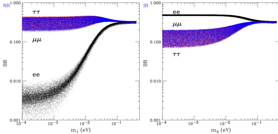
Figure 4-10. H^{\pm\pm} decay branching fractions as a function of the lightest neutrino mass, assuming a normal (left) or inverted (right) neutrino mass hierarchy. See [?] for details.
