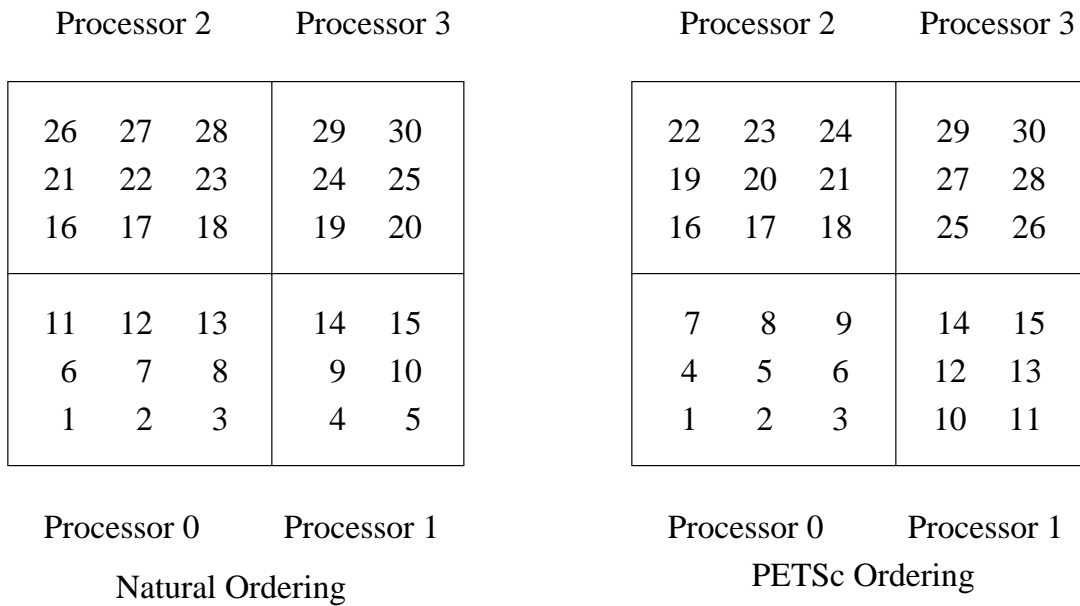
Figure 8: Natural Ordering and PETSc Ordering for a 2D Distributed Array (Four Processes)
