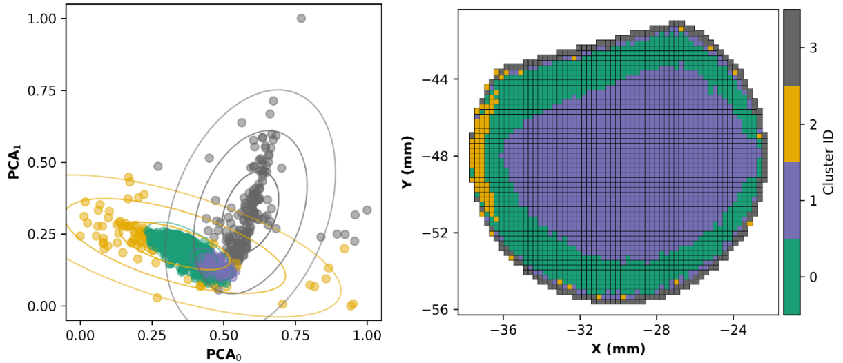
Figure 7. Cluster analysis of simulated melt pool characteristics in a 3D printed stainless steel.
