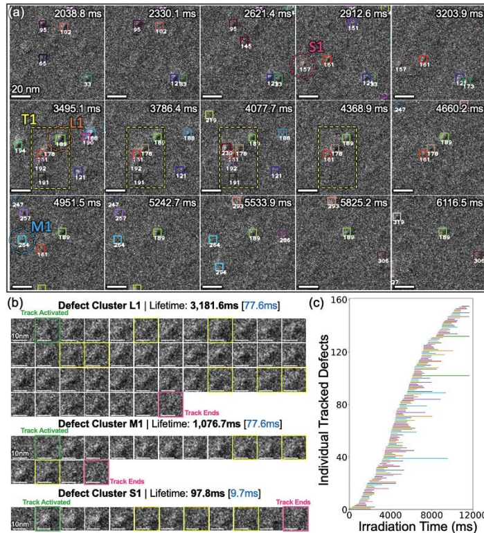
Figure 9. Visualization of the DefectTrack 's multi-object tracking performance on a representative test set of TEM video data showing formation and annihilation of defect clusters during in situ ion irradiation. [24]
