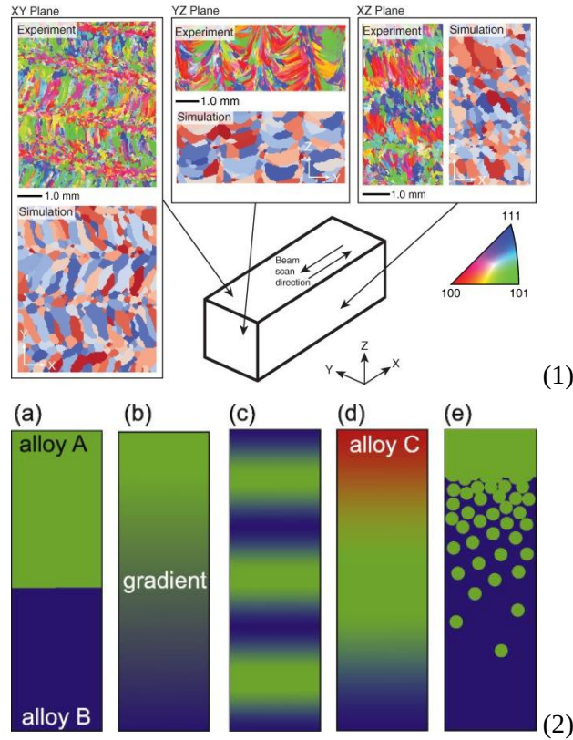
Figure 1. (1) spatially heterogeneous microstructures of an additively manufactured alloy revealed by experiments and modeling [4]; (2) composition of different alloys to form functionally graded parts [5].
